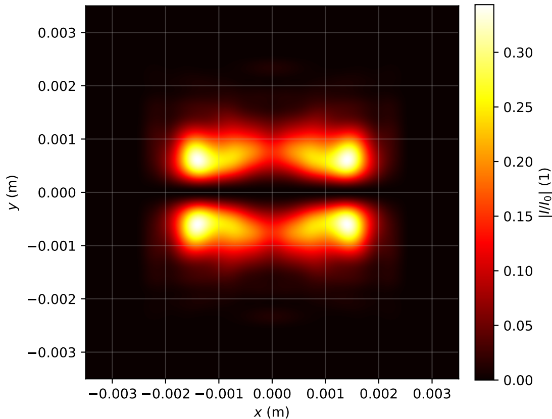
Intensity profile I(x, y, z = 3.184)/I_0 , P_{in}=4.0P_{cr} , artificial time
